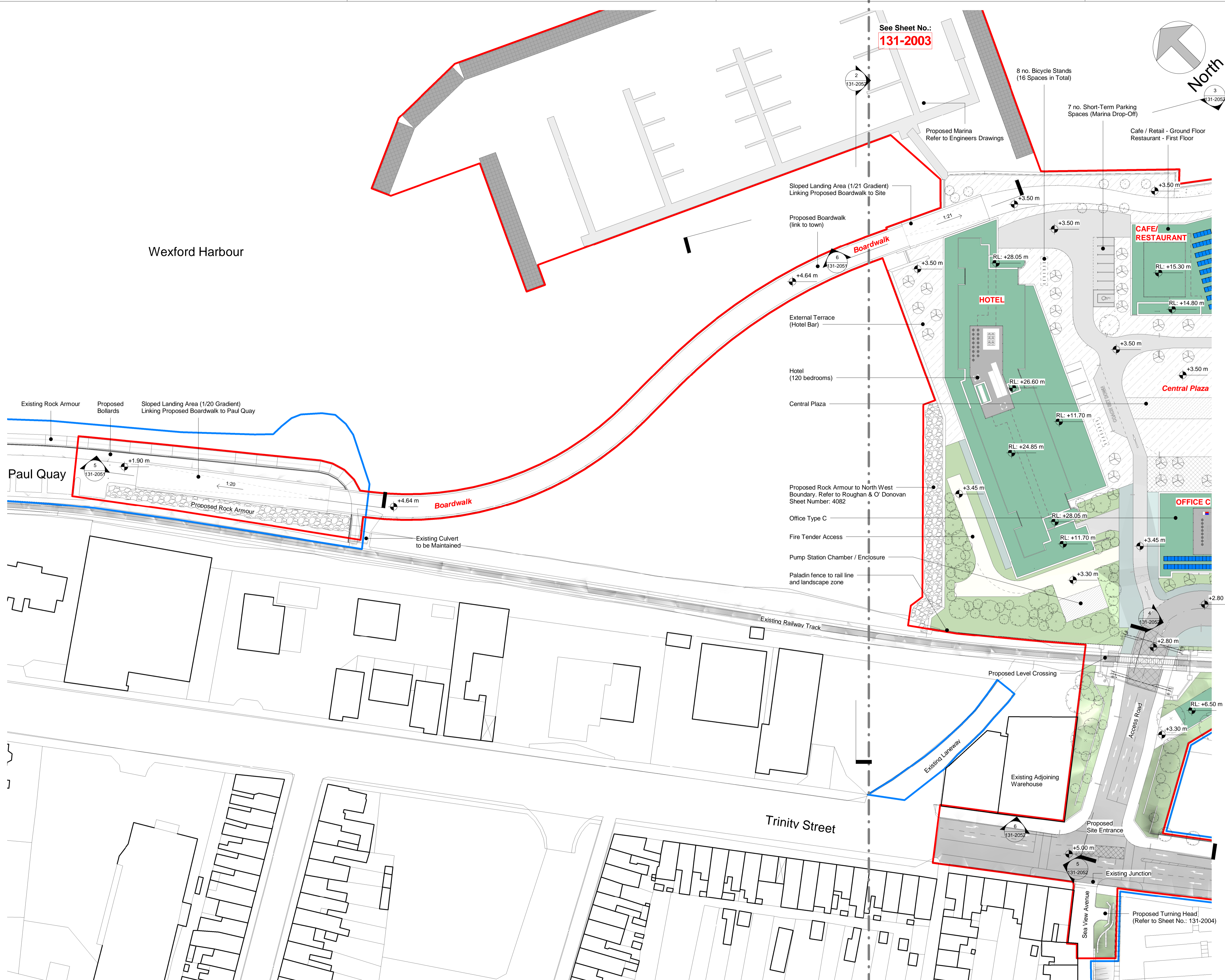
1-PROPOSED SITE LAYOUT - PAUL QUAY & BOARDWALK 1 : 500
